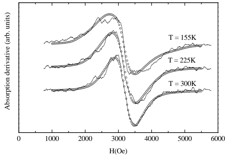
Figure 6. Low-temperature evolution of the HT EPR spectra. The dotted curves are fits using the same anisotropy, average volume, and dispersion for the three temperatures. The observed narrowing on increasing T is due to the dynamics of the superparamagnetic behaviour.
